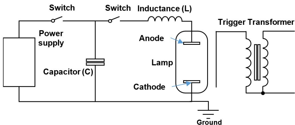
Fig. 1. Schematic diagram of intense pulsed light system.
